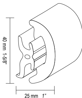
RADIAL 40
