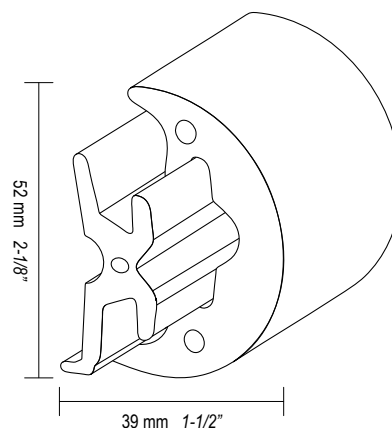
RADIAL 52
