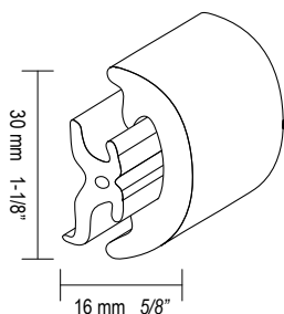
RADIAL 30
